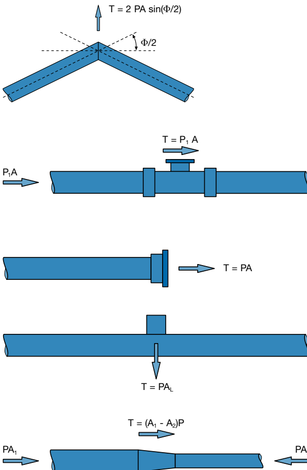
Figure 10-5 Schematic View of Concrete Reaction
