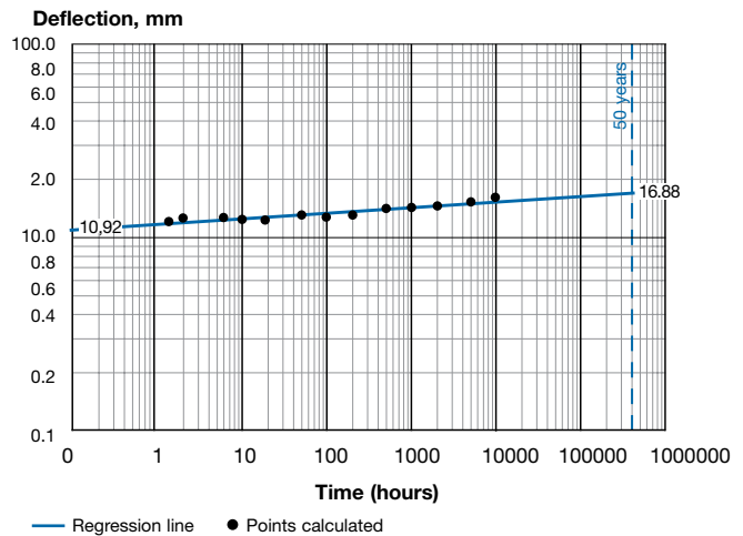
Figure 5-6-7 Long Term Stiffness SN 5000 PN 16
