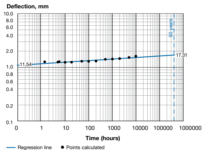
Figure 5-6-8 Long Term Stiffness SN 5000 PN 6
