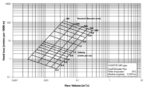
Figure 6-11-1 Head Loss – Small Diameters
