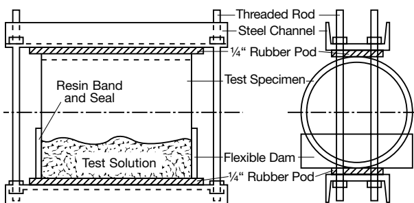
Figure 5-6-1 Strain Corrosion Test Apparatus
