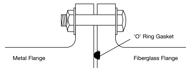
Figure 8-1-1 Flanged Joint
