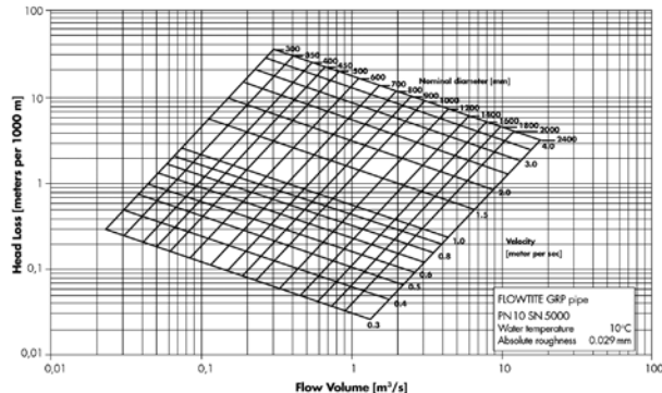
Figure 6-11-2 Head Loss – Large Diameters
