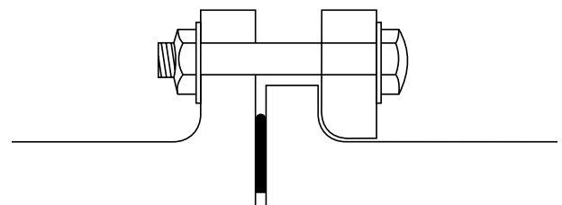
Figure 8-1-3 Loose Ring with Flat Gasket incl. Steel Support
