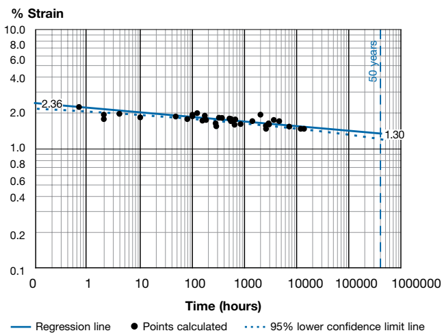
Figure 5-6-6 FLOWTITE Line for Long Term Bending
