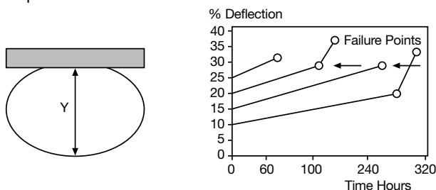
Figure 5-6-5 Effect of Long Term Bending in Water in Pipe Life
