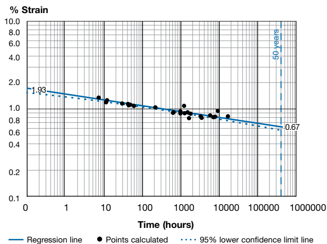
Figure 5-6-2 FLOWTITE Line for Strain Corrosion
