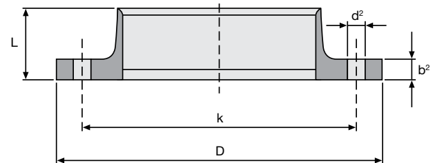
Figure 8-1-2 Fixed Flanged Joint
