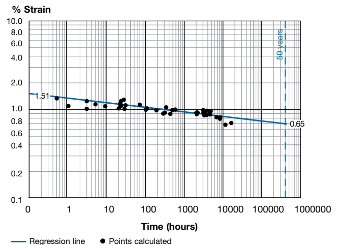
Figure 5-6-4 FLOWTITE Line for Long Term Pressure Strain
