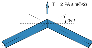
Figure 10-9 Thrust Force
